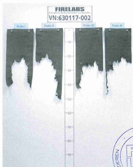
fig. 4 View of test specimen after the test
