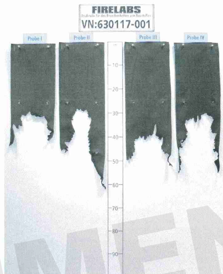
fig. 2 View of test specimen after the test
