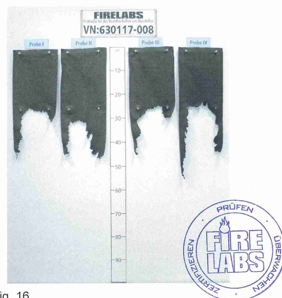
fig. 16 View of test specimen after the test
