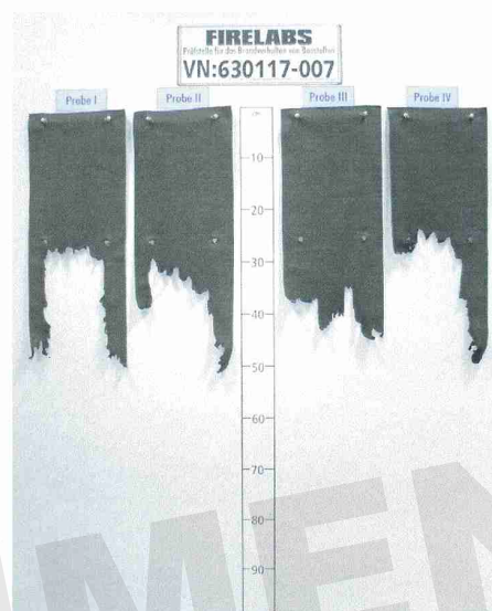
fig. 14 View of test specimen after the test
